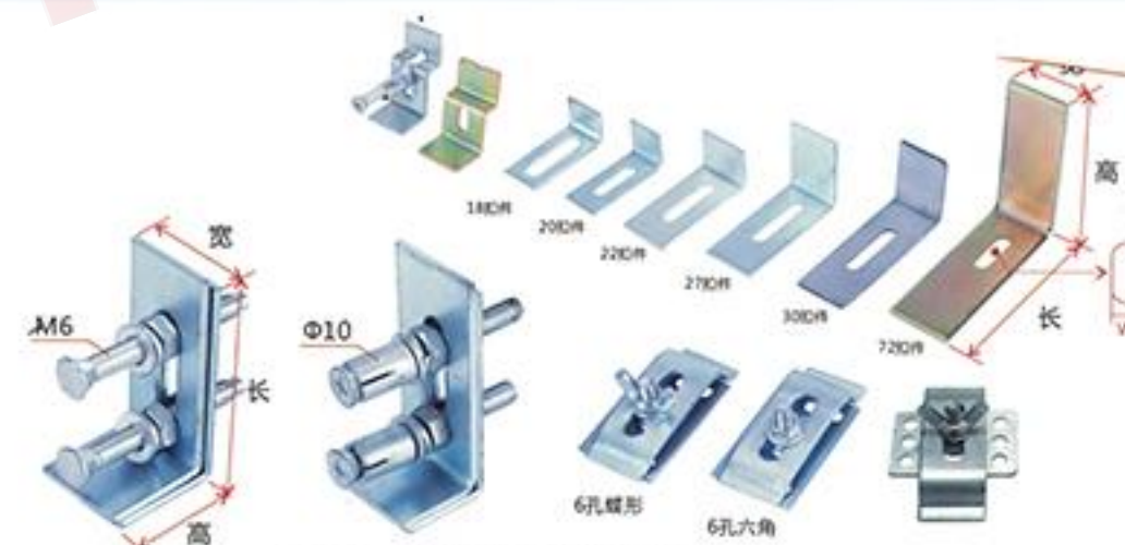
OSA-151 台下盆扣件 Basin connector under the counter
