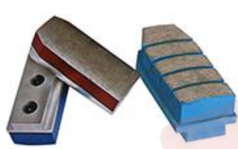
AT-07 金刚布拉磨块 Diamond fickert brick for granite 规格 Specification: L140, L170 Grit: 36#, 46#, 60#, 80#, 120#
