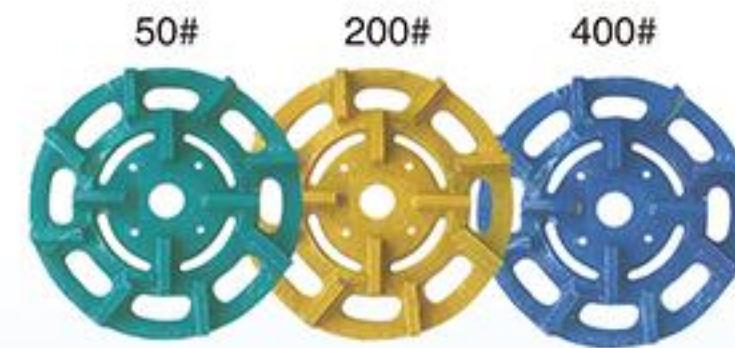
AT-15 金属磨盘 Metal grinding plate 规格 Specification: 8" (175mm) 10" (215mm) Grit: 50#, 200#, 400#
