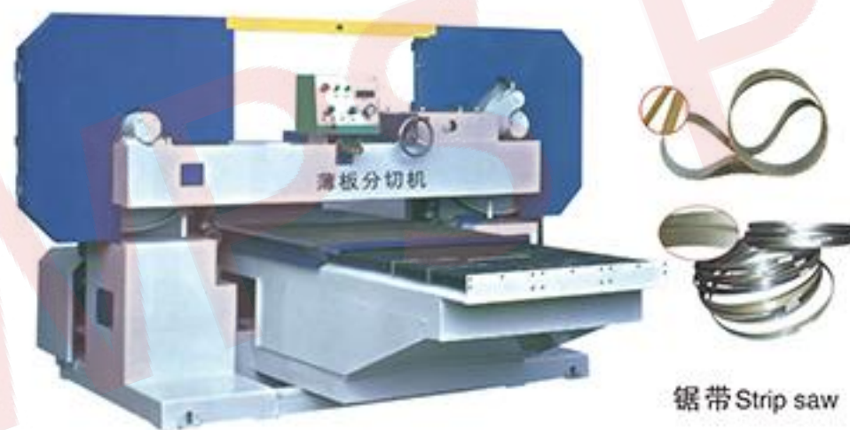
M-27 大理石薄板分切机 Marble Sheet Metal Cutting Machine
