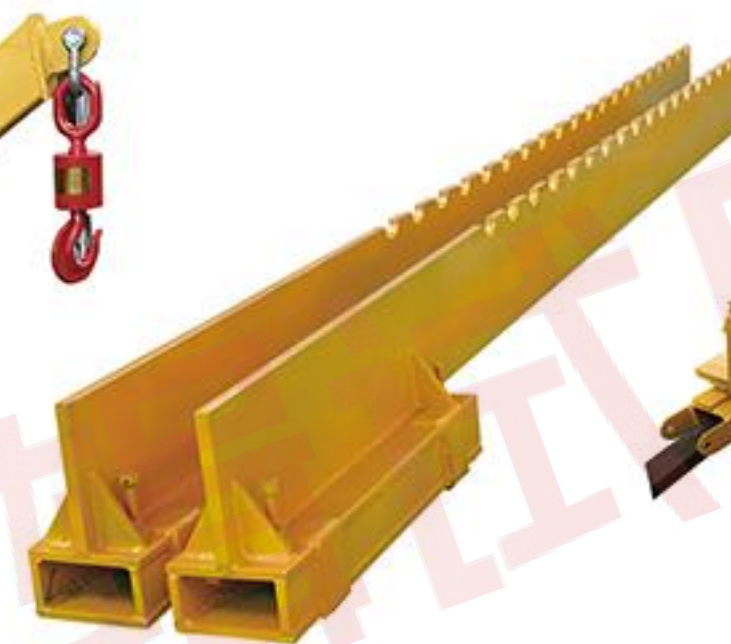
SE-41 铁板款叉车加长吊臂 Forklift lengthened boom 长:5400mm 宽:250mm 高:400mm 承重: 5t
